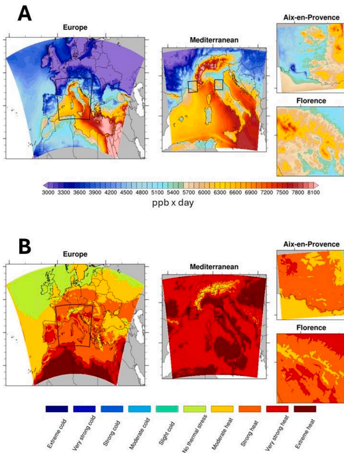
Fig. 9. Maps of SOMO35 (upper panel) and thermal heat stress (UTCI, lower panels) over the different domains as simulated by WRF-Chem for the year 2019.
